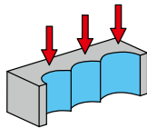
Chain drilling
