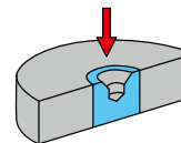
Spot drilling in a central hole
